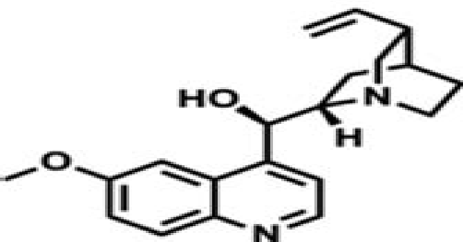
Quinine (QN)
