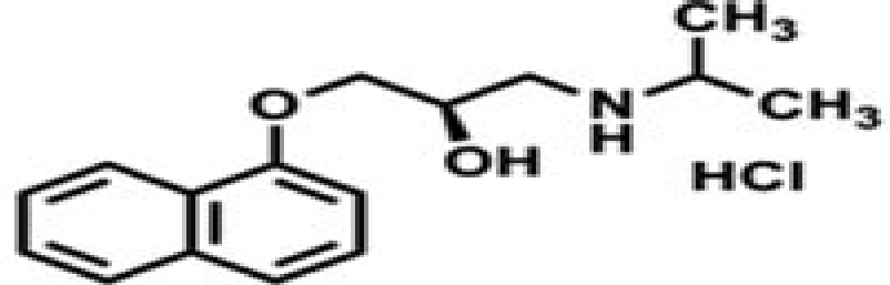
(R)-(+)-Propranolol
