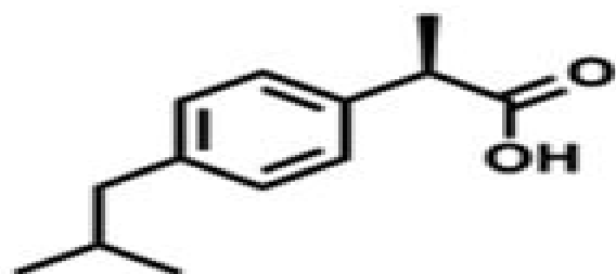
(R)-(-)-Ibuprofen
