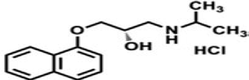
(S)-(-)-Propranolol
