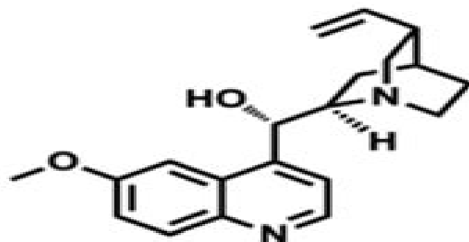
Quinidine (QND)
