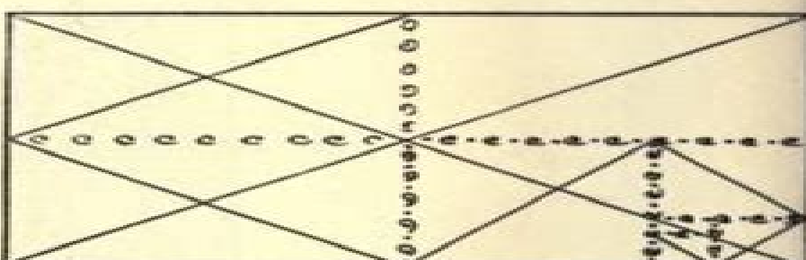
LAYOUTS IN THE WHIRLING SQUARE ROOT
