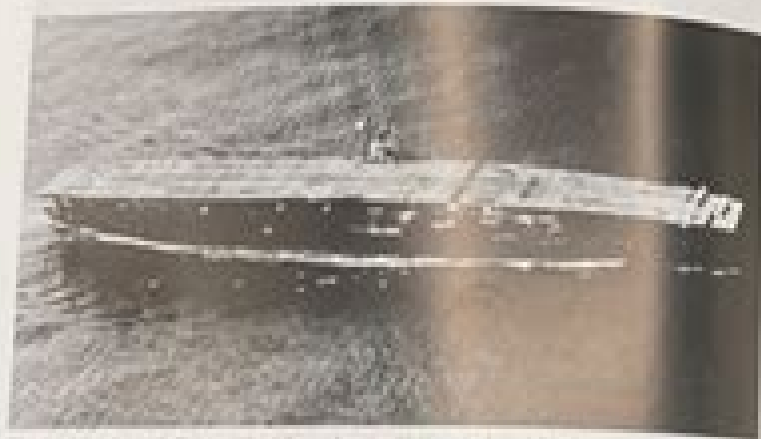
The Japanese aircraft carrier Akagi (CV-6) shown here in 1941 with three Mitsubishi A6M Zero fighters pulled forward. Akagi was sunk on 4 June 1942 after being fatally damaged by US aircraft during the Battle of Midway (NARA, 800-500-0000).
