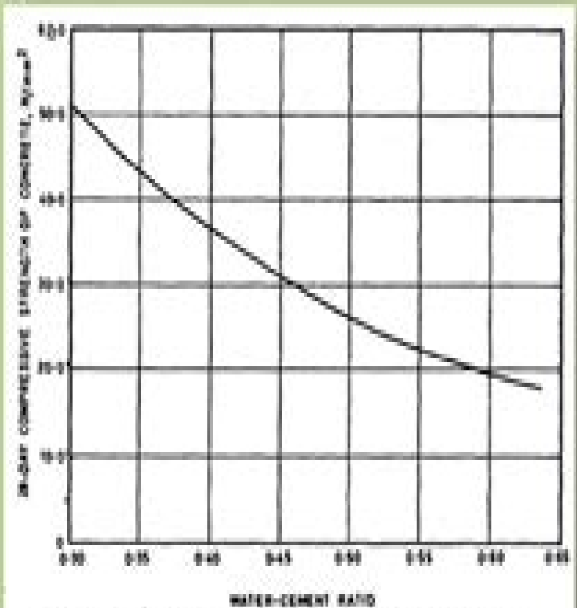
FIG. 1 GENERALISED RELATION BETWEEN FREE WATER-CEMENT RATIO AND COMPRESSIVE STRENGTH OF CONCRETE
