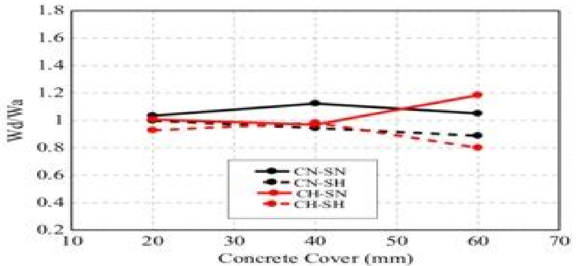
Fig. 14 Comparison of crack width in case of concrete cover
