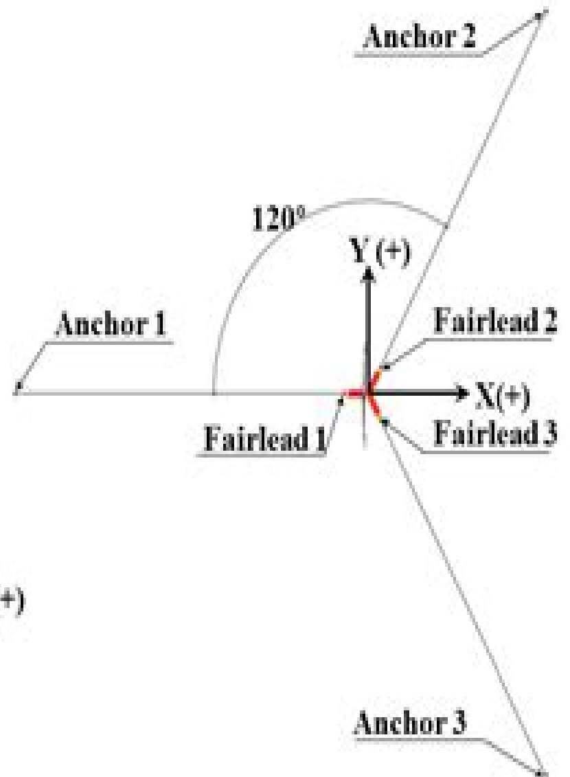
(b) Mooring system arrangement
