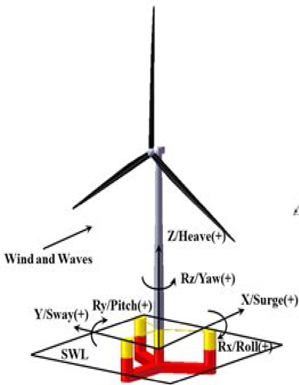
(a) Reference coordinate system of wind turbine
