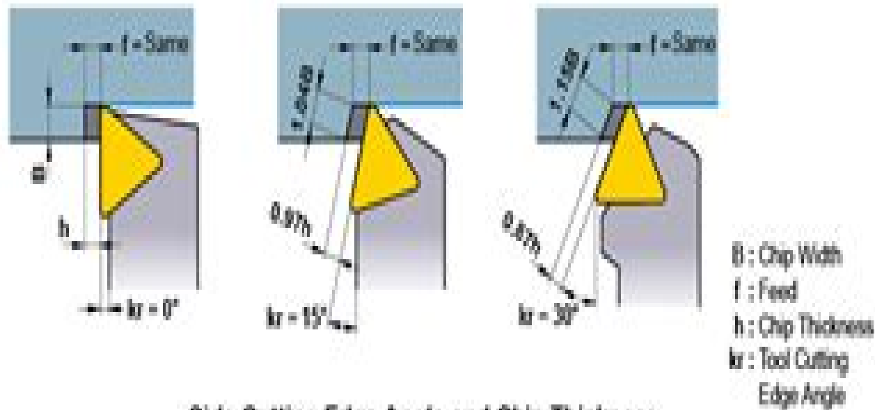
Side Cutting Edge Angle and Chip Thickness
