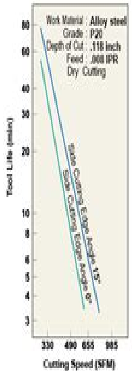
Side Cutting Edge and Tool Life
