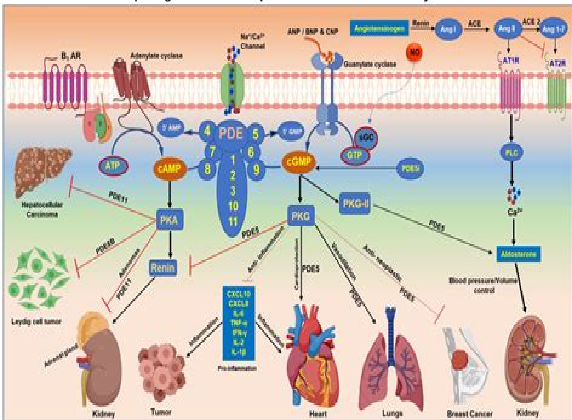
Schematic illustration depicting the role of Phosphodiesterases in Endocrine system and related diseases
