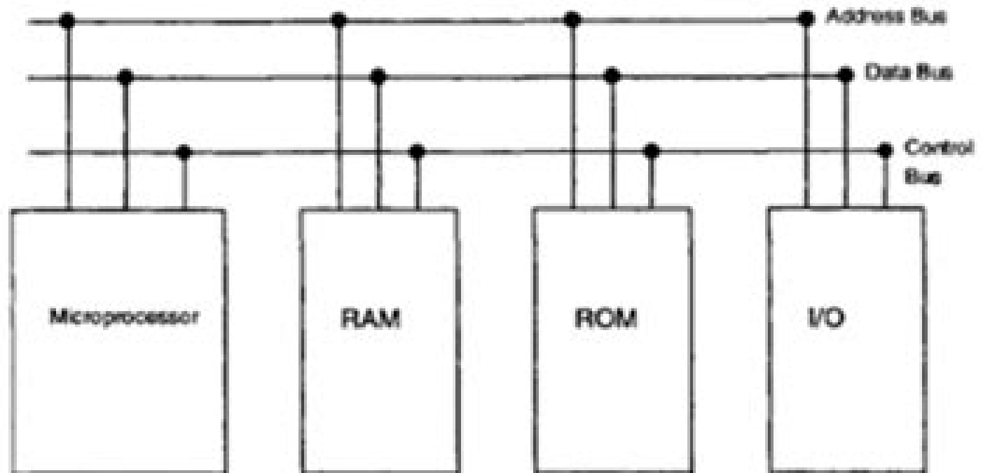
FIGURE 6.2 Simplified version of a typical microcomputer
