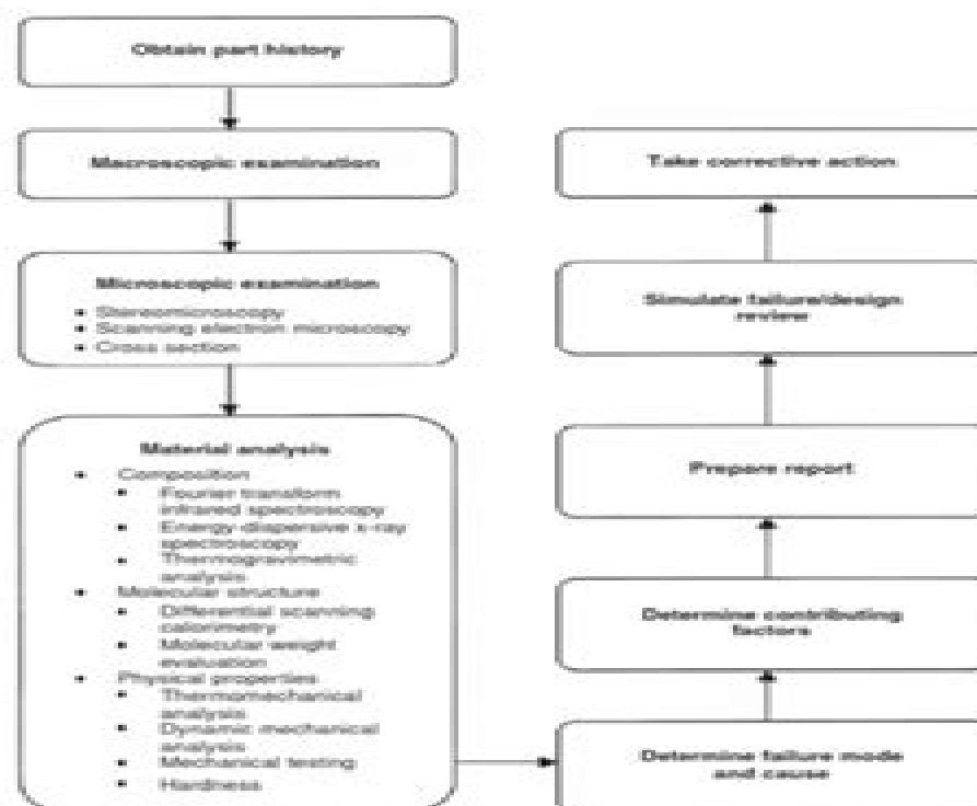
Fig. 1 Steps for performing failure analysis. The steps are the same regardless of the material.
