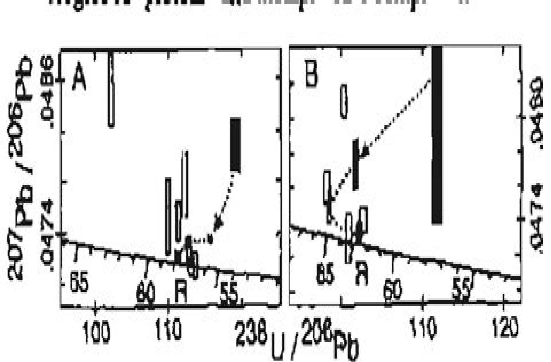
Figure 1. Tera-Wasserburg diagrams showing conventional
