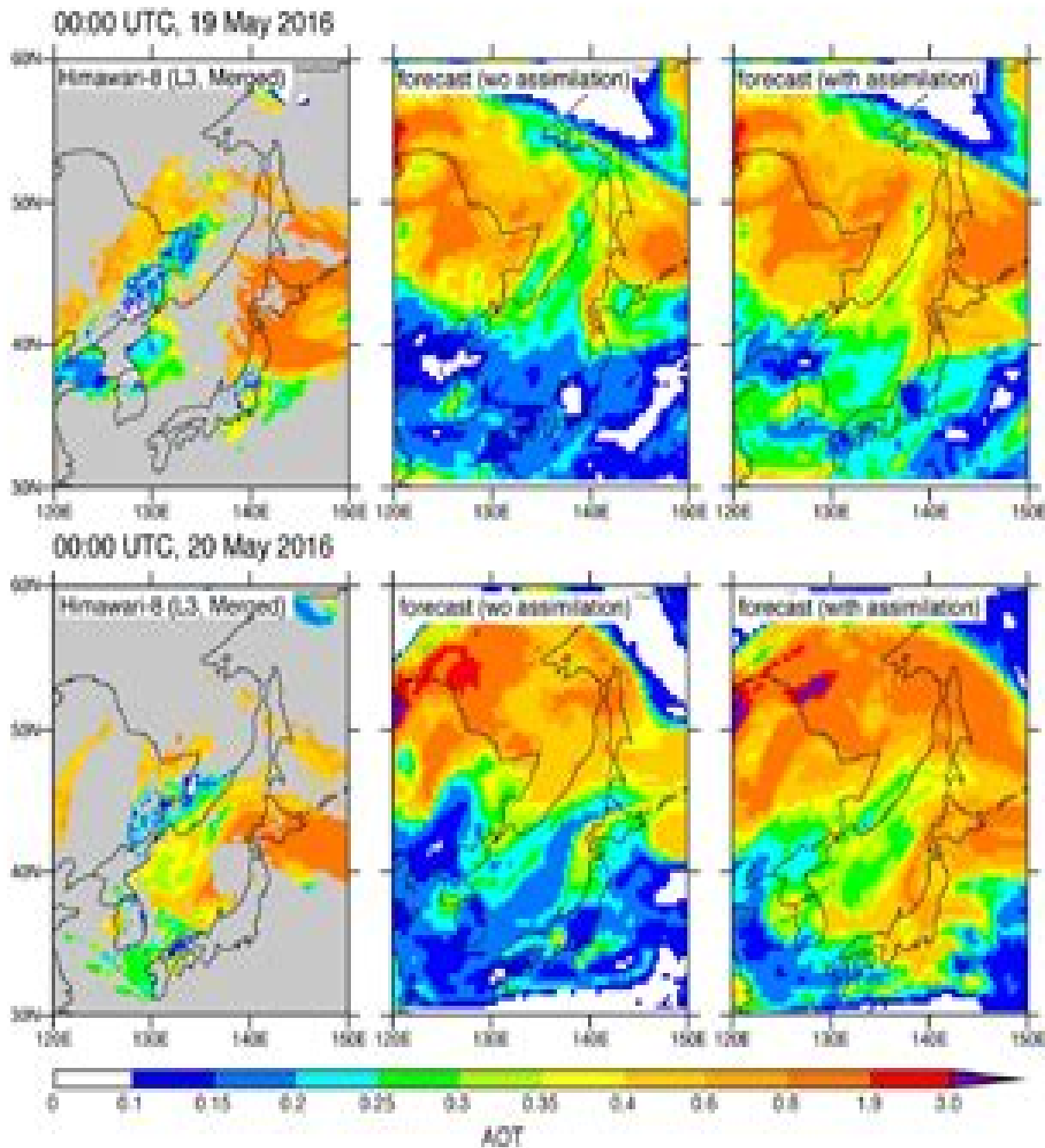
←Figure 1. Horizontal distribution of observed and forecasted aerosol optical thickness (AOT) on May 19 (upper panels) and May 20 (lower panels), 2016: (left panels) observed from Himawari-8, (central panels) forecasted without data assimilation, and (right panels) forecasted with data assimilation.
