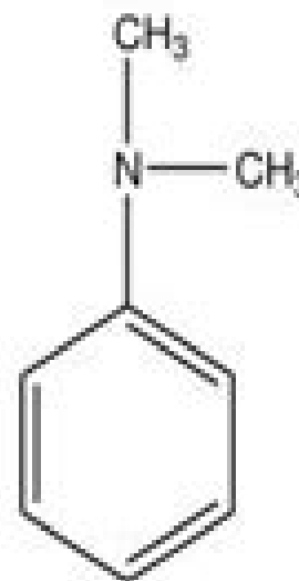
N,N -dimethylbenzenamine
