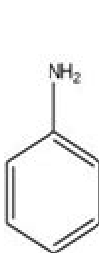
aniline
