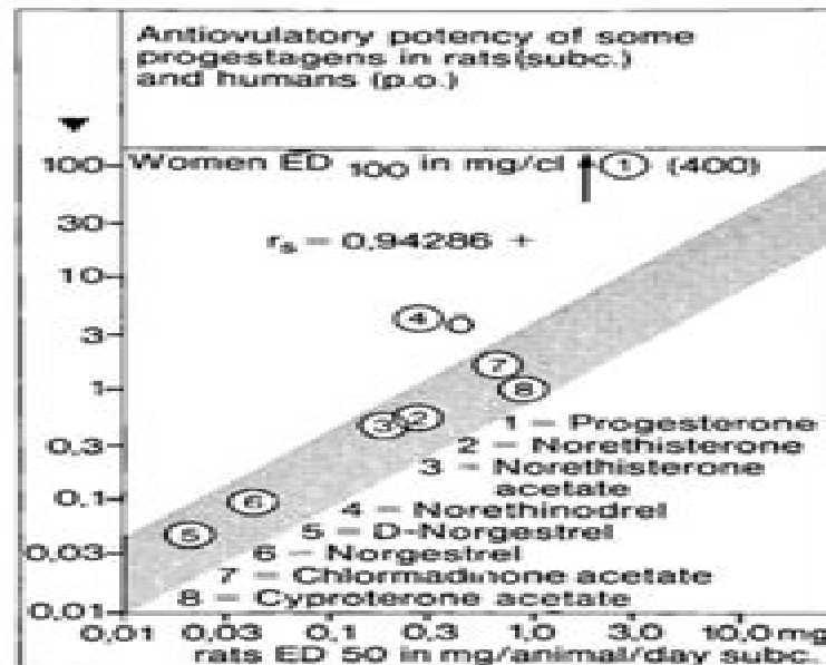
Fig. 10 Antiovarulatory efficacy of various progestins. Comparison of the oral ovulation-inhibiting dose in women with subcutaneous doses in rats.
