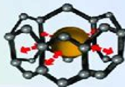
Host-Guest interaction
