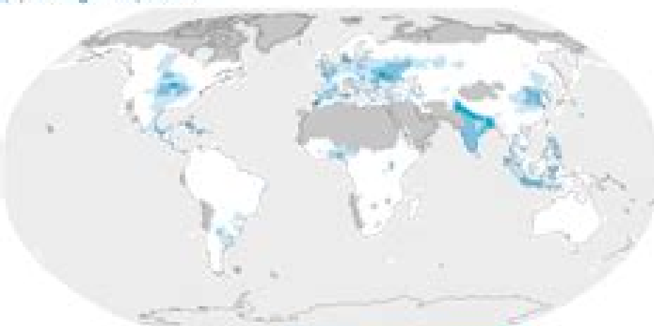
(c) Drought exposure
