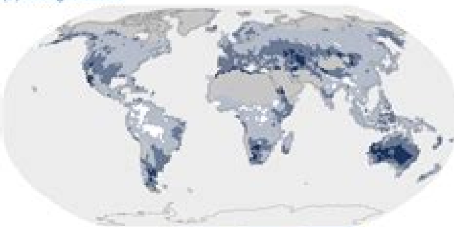
(a) Drought hazard
