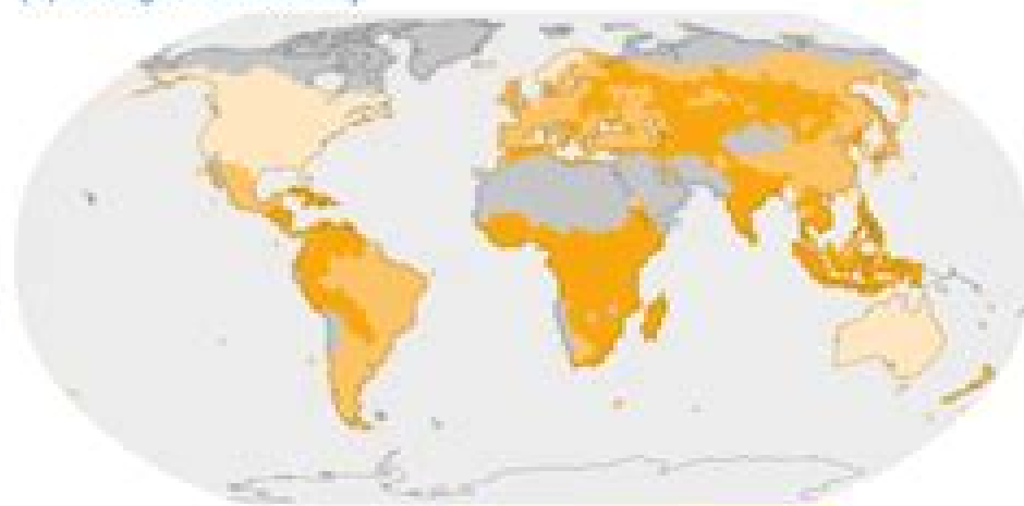
(b) Drought vulnerability
