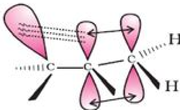
Fig. 12.4(b) Orbital diagram showing hyperconjugation in propene
