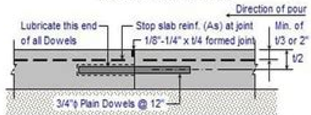
Typical Construction Joint for Load Transfer
