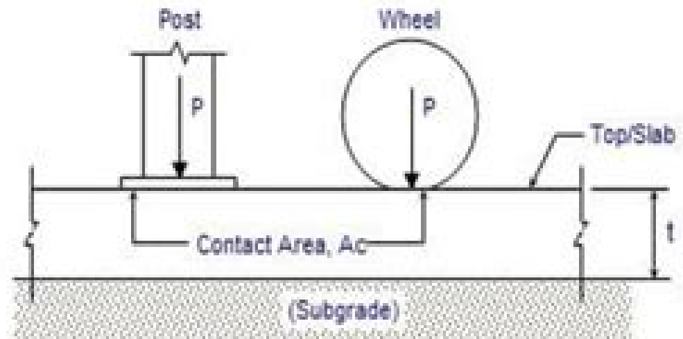
Concrete Slab on Grade
