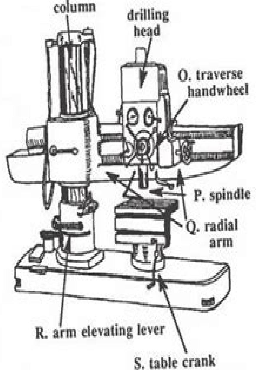
T. Radial Drilling Machine
