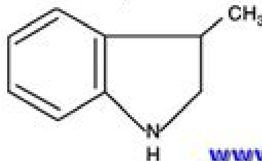
3-methyl indol
