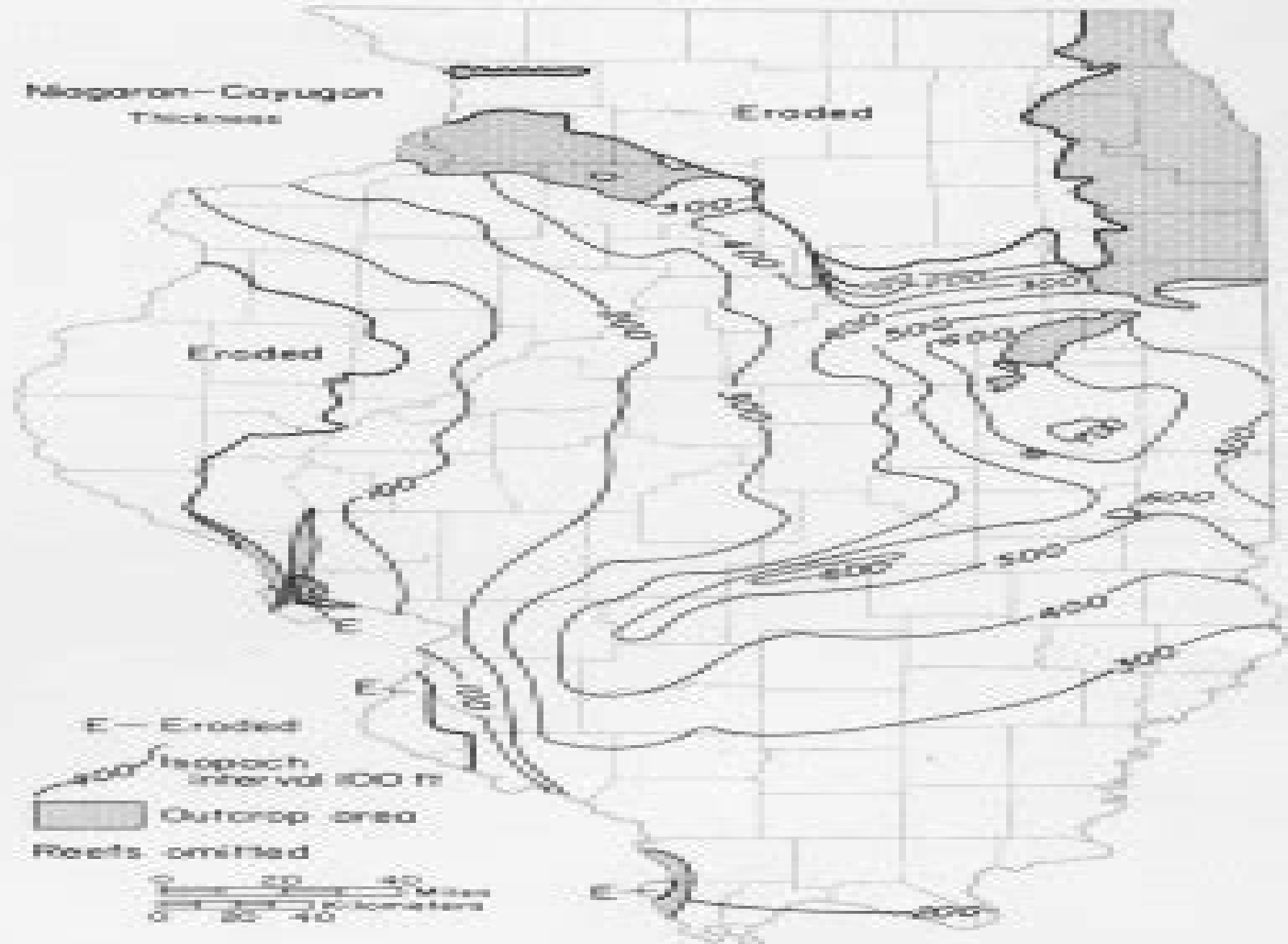
Fig. S-15—Thickness of the Niagara Series; includes the Cayuga Series in southern Illinois.
