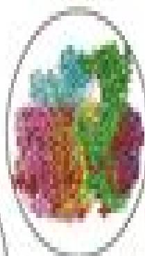
Cryo-Electron Microscopy
