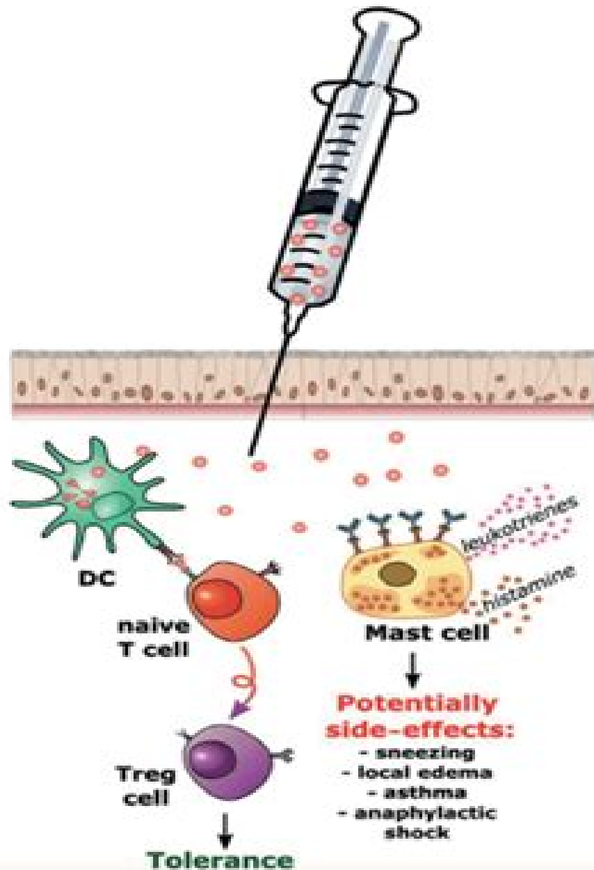
(A) AIT with soluble allergen
