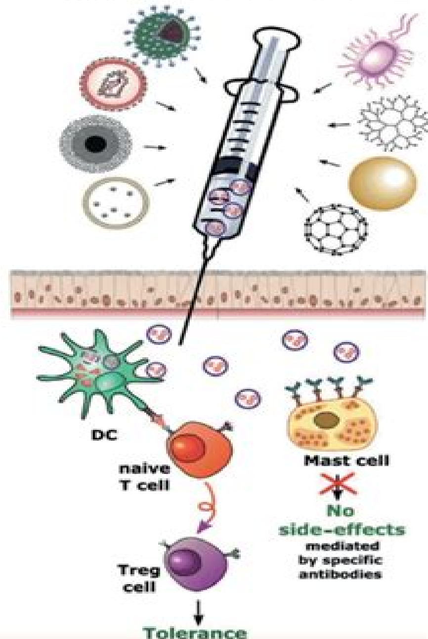
(B) AIT with allergen encapsulated in NPs
