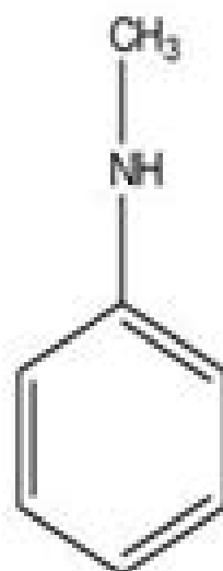
N -methylbenzenamine
