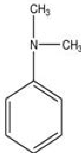
N,N -dimethylbenzenamine
