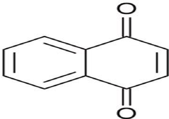
1,4-naphthoquinone
