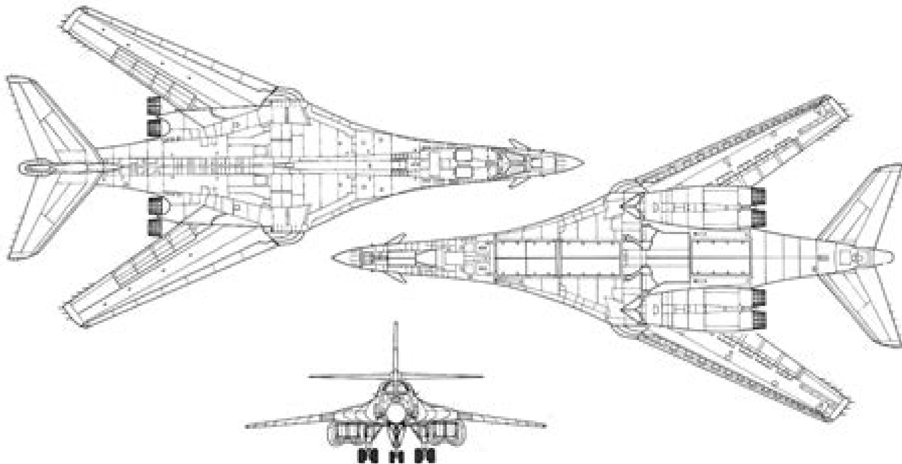
Rockwell B-1B Lancer
