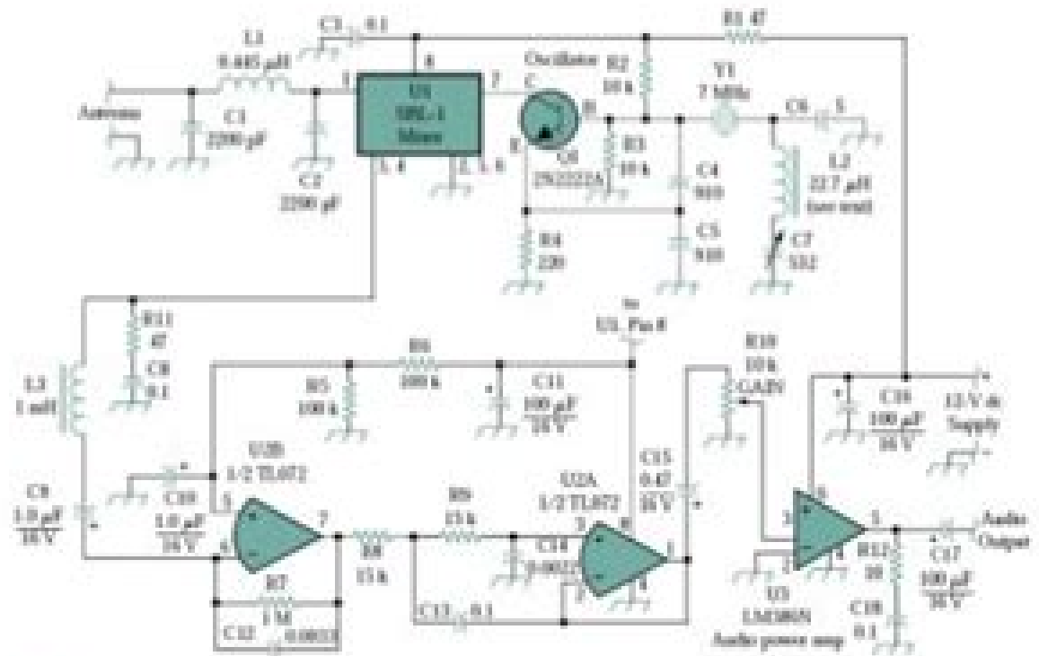
Figure 1.2 Electric circuit of a radio receiver. (Reproduced with permission from NYT , August 1960, p. 21.)
