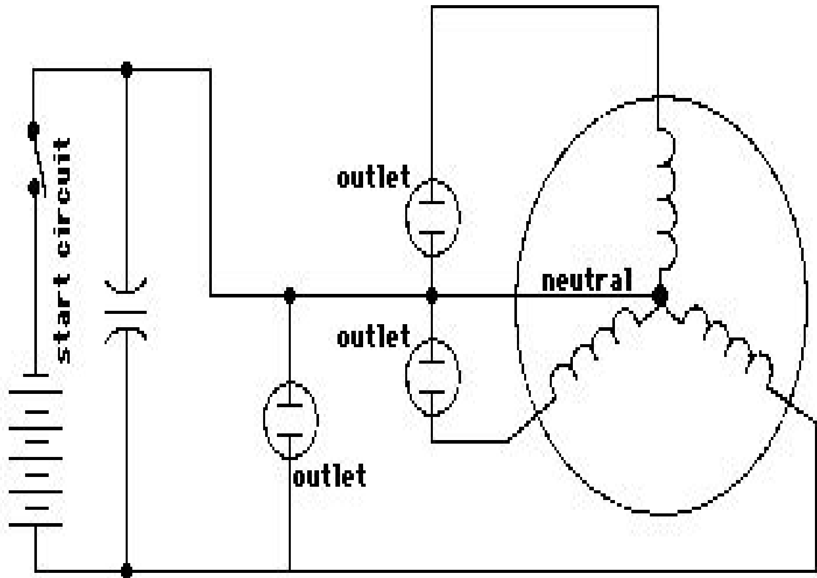
THREE PHASE STAR MOTOR WITH NEUTRAL each outlet delivers 220 VAC at 60 Hz
