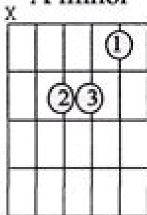
A minor
