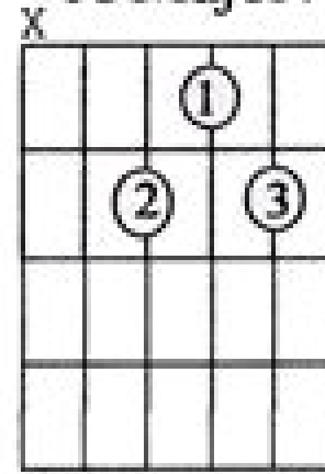
A Major7
