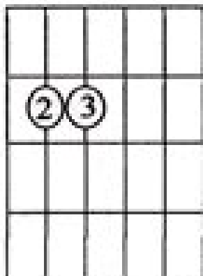
E minor
