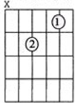
A minor7
