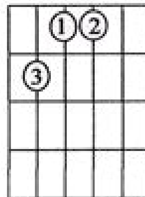
E Major7
