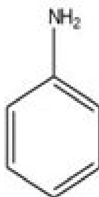
aniline
