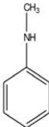
N -methylbenzenamine
