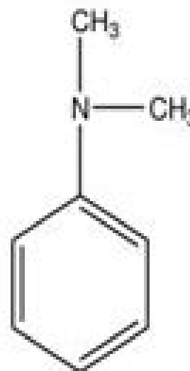
N,N -dimethylbenzenamine
