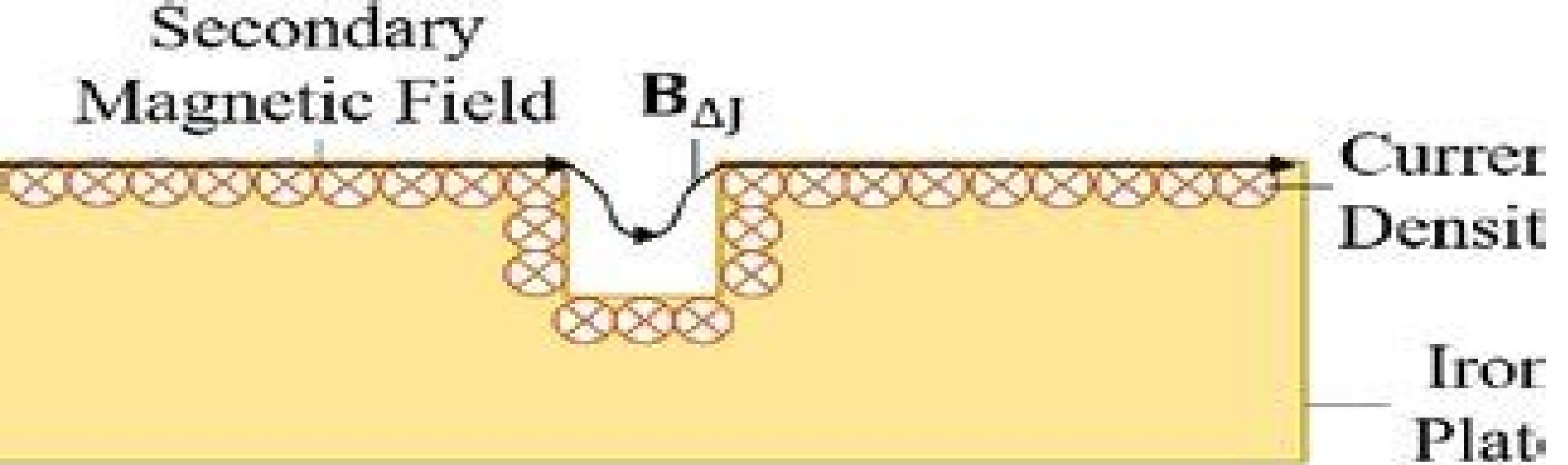
(a) The distribution of B_{\Delta J}
